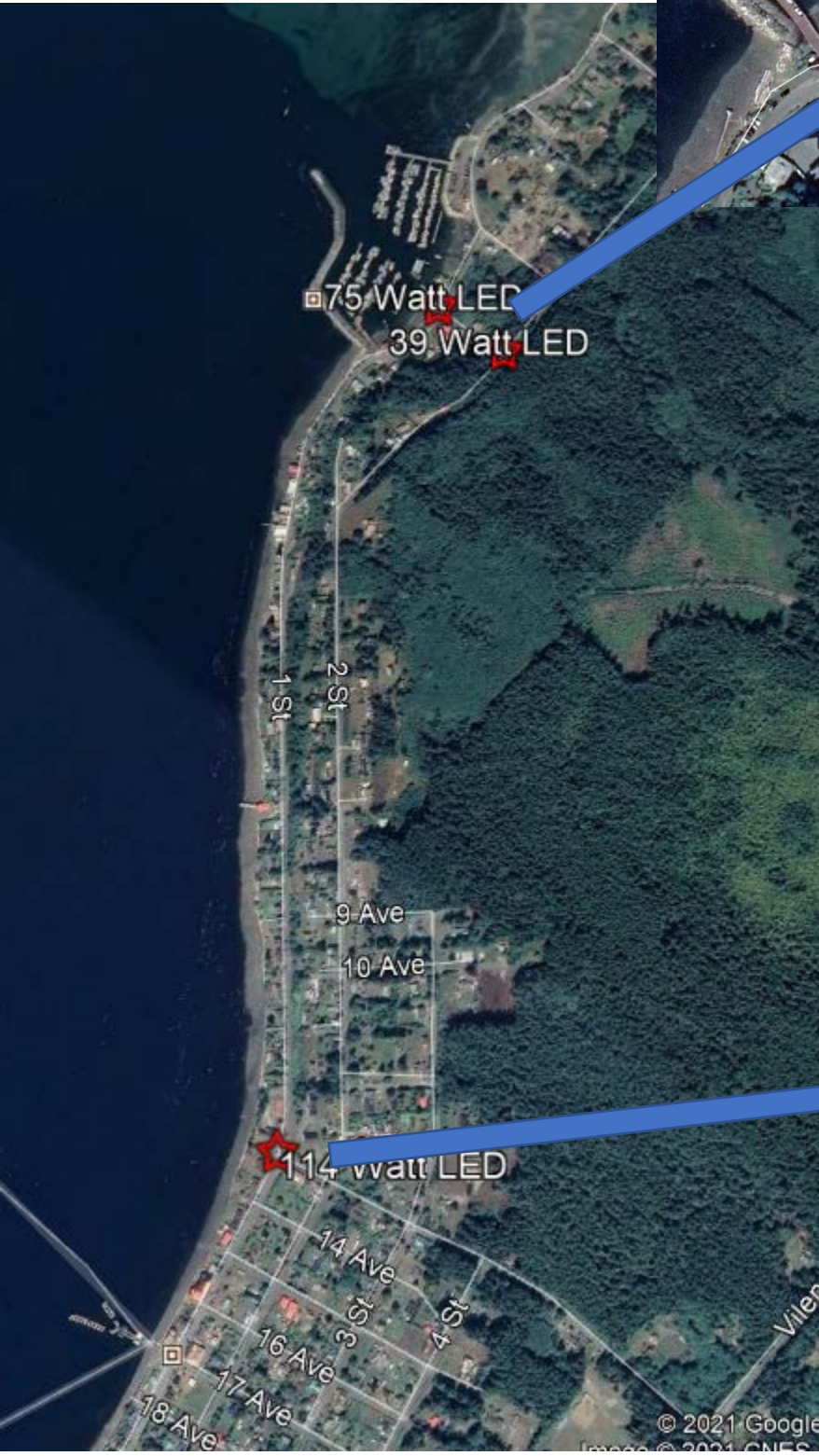
Location Map of Installed LED Street Lights in Sointula as of April 19, 2021
